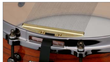
42 strands Regular Hi-Carbon Steel snare wires
